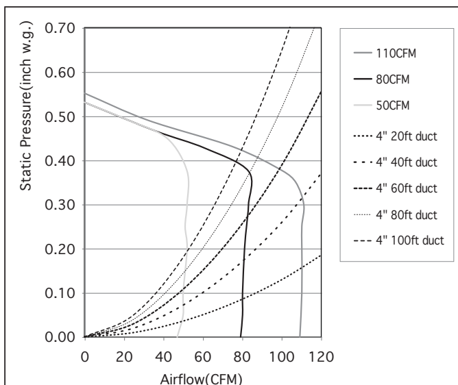
Performance Curve FV-0511VFL1K - 4" Duct
